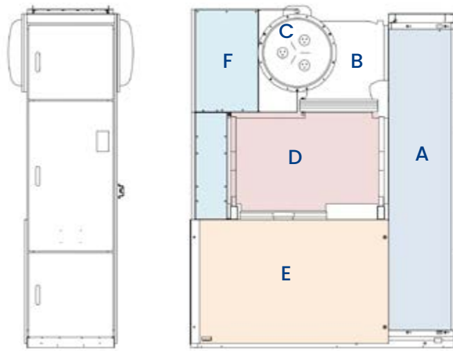
BGP-40.5 compartments
