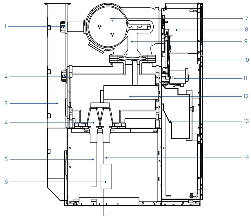
BGP-40.5 standard structure
