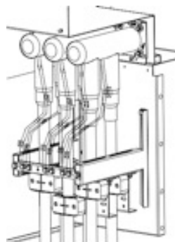
Two cables per phase (only available in the TGS 1,432 mm height version)
