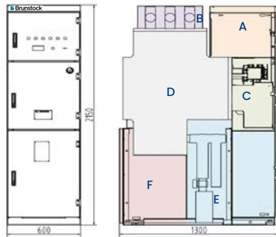
BGS-40.5 compartments
